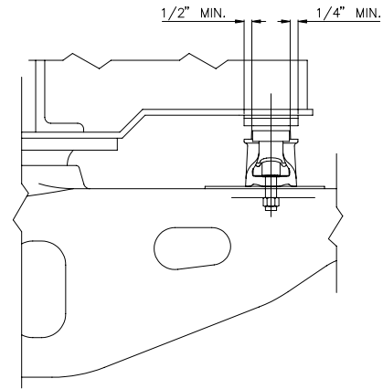
Figure 4. Minimum Plate or Wedge Overhang
