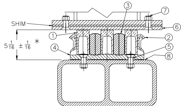
Figure 5. 690-RL Side Bearing Arrangement
